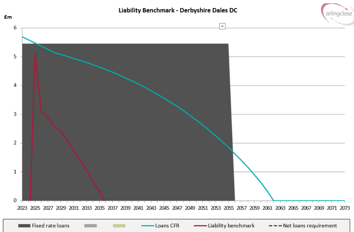
Chart 1: Liability Benchmark
